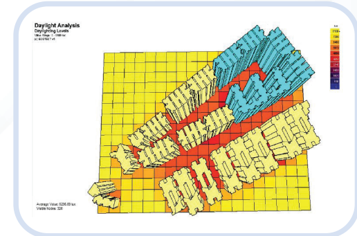
Daylight Analysis
