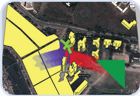
Shadow Analysis
