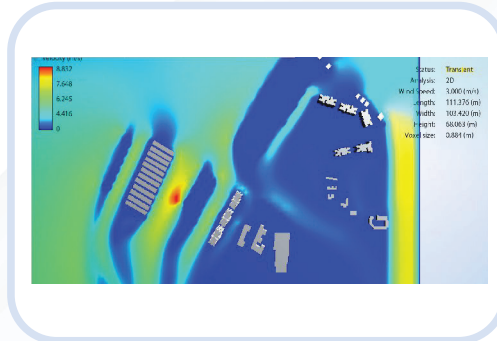
Wind Analysis
